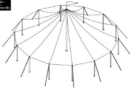
ISOMETRIC VIEW 140m 2 1-Mast Sailcloth Zelt
