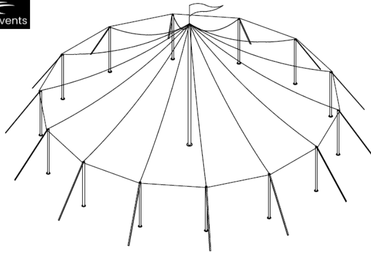
ISOMETRIC VIEW
