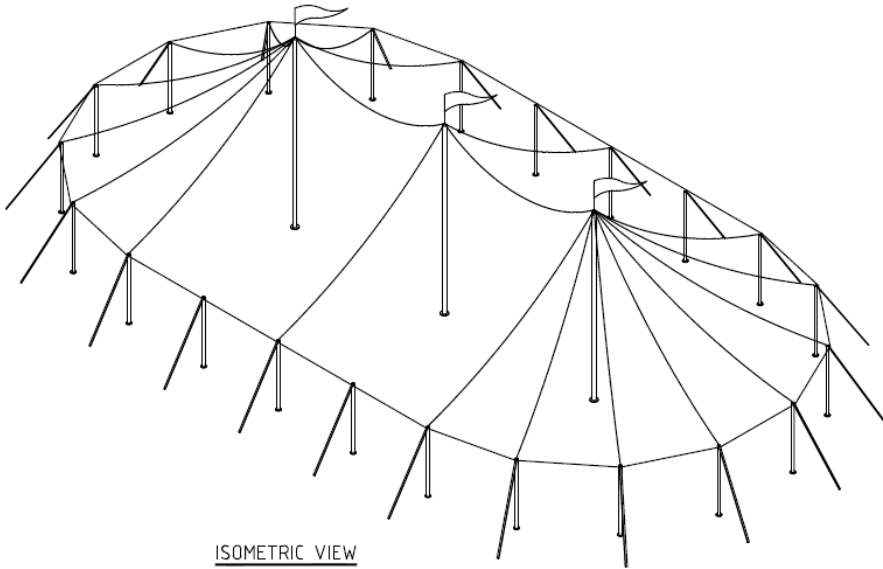
ISOMETRIC VIEW
